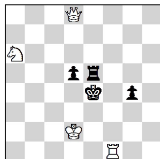
18. #2 4 + 4 Meson No. 4702
