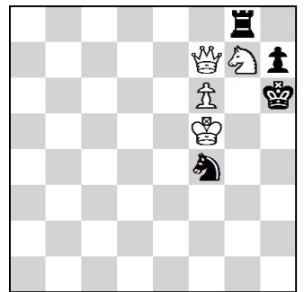
12. #2 4 + 4 Meson No. 78111
