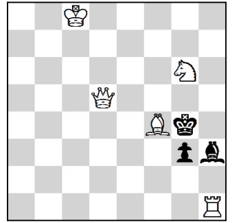
4. #2 5 + 3 Meson No. 132067
