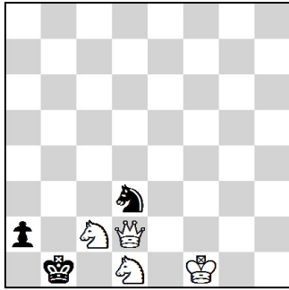
5. #2 4 + 3 Meson No. 7442
