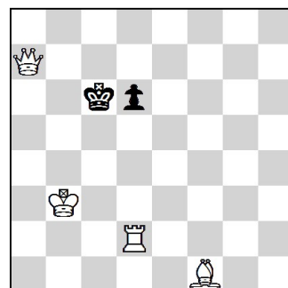
19. #2 4 + 2 Meson No. 6617
