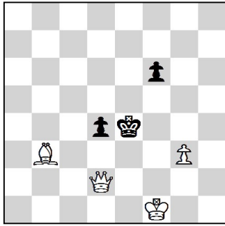
1. #2 4 + 3 Meson No. 4739
