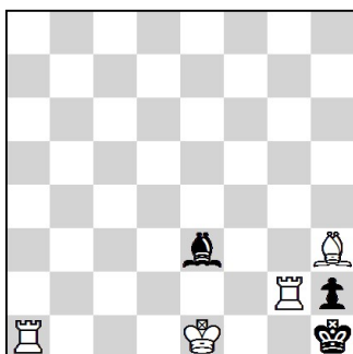
17. #2 4 + 3 Meson No. 23443
