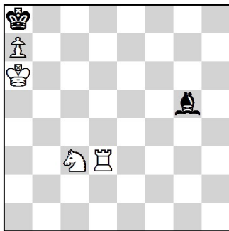
9. #2 4 + 2 Meson No. 22337
