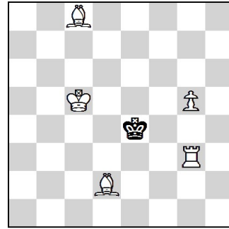
7. #2 5 + 1 Meson No. 1953
