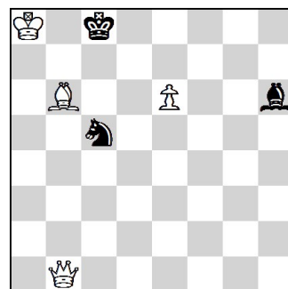
15. #2 4 + 3 Meson No. 15791
