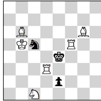
6. #2 6 + 3 Meson No. 157319
