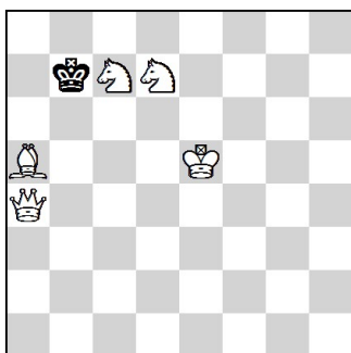
13. #2 5 + 1 Meson No. 227094
