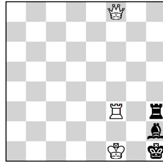
3. #2 3 + 3 Meson No. 195059
