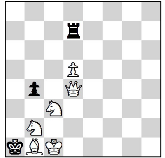
8. #2 6 + 3 Meson No. 787
