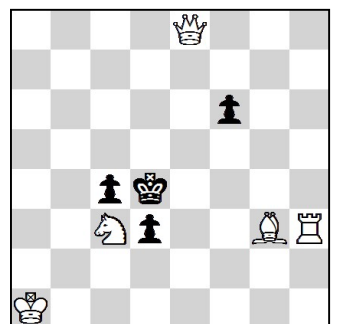
20. #2 5 + 4 Meson No. 51607
