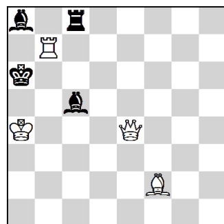
14. #2 4 + 4 Meson No. 157145
