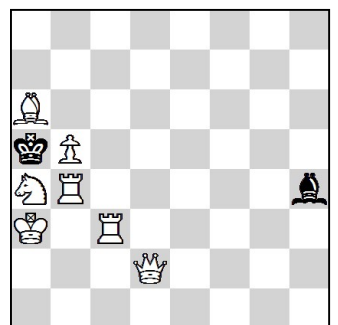
16. #2 7 + 2 Meson No. 10058
