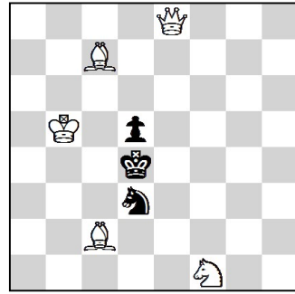
2. #2 5 + 3 Meson No. 4939
