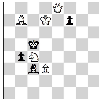
10. #2 5 + 4 Meson No. 79019
